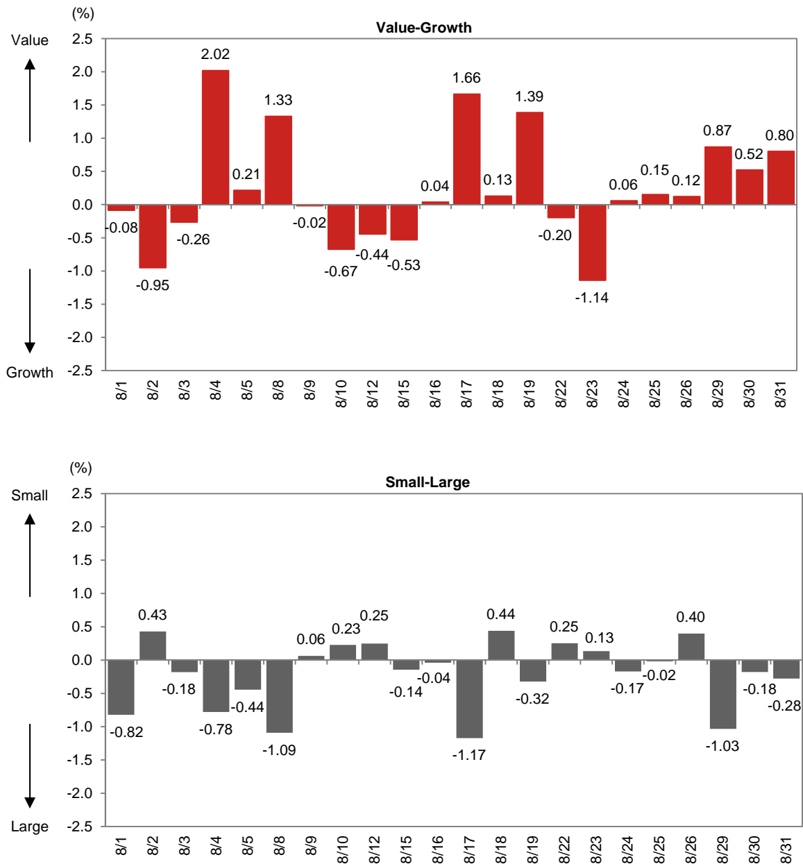
Fig. 7: Daily performance
