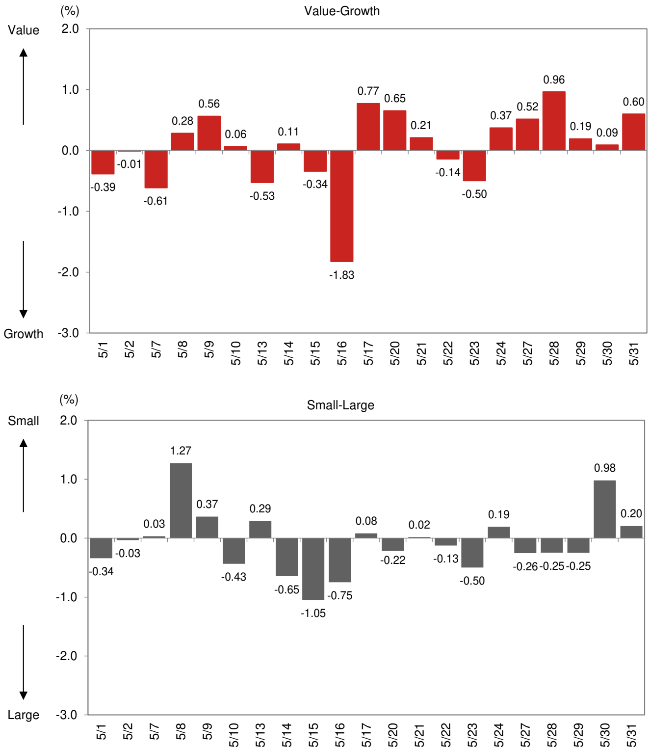
Fig. 7: Daily performance
